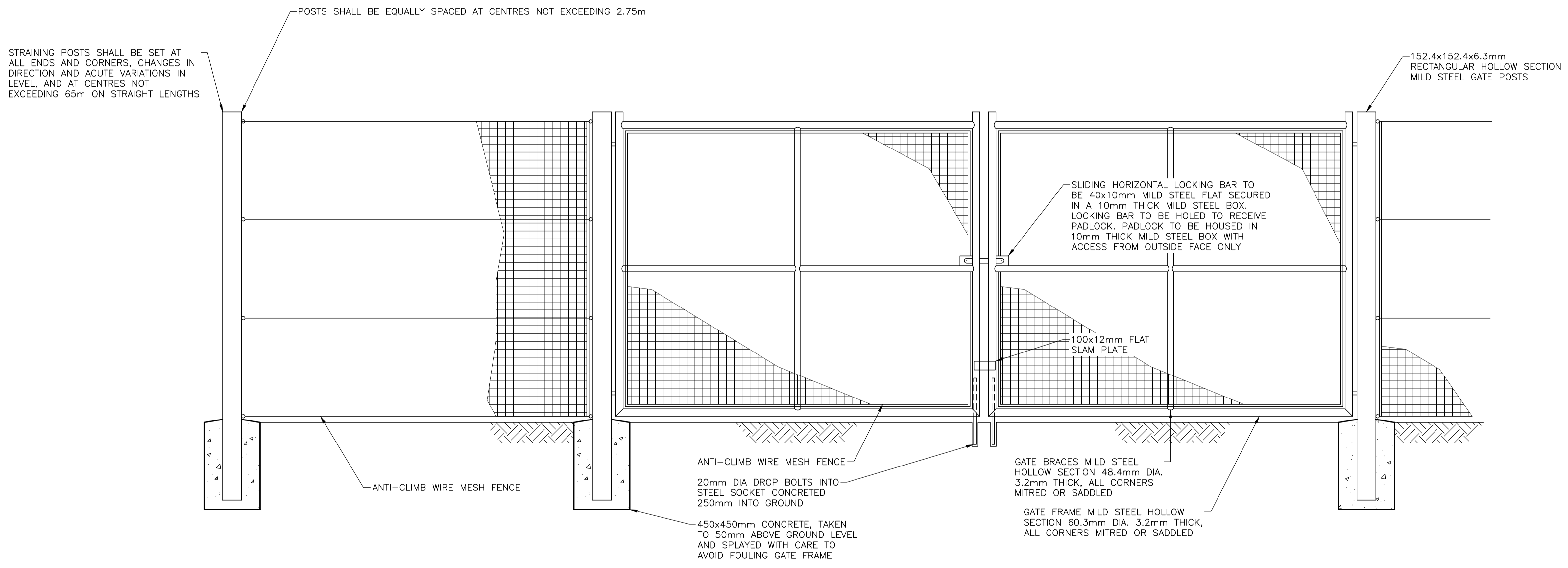
GREEN WELDED MESH FENCE & GATE DETAIL SCALE 1:20
